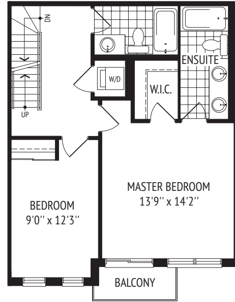
THIRD FLOOR
